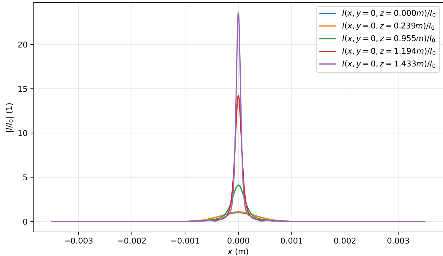
Intensity profile I(x, y = 0, z)/I_0 , Pin=1.8Pcr, artificial time
